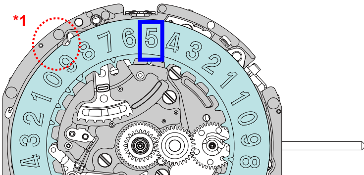
Pillar in main plate at 11 o'clock position
